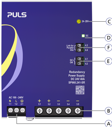
Fig. 14-1: Front side
