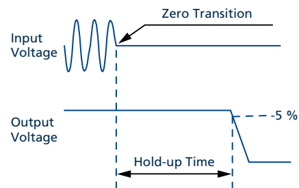
Fig. 7-2: Shut-down behaviour
