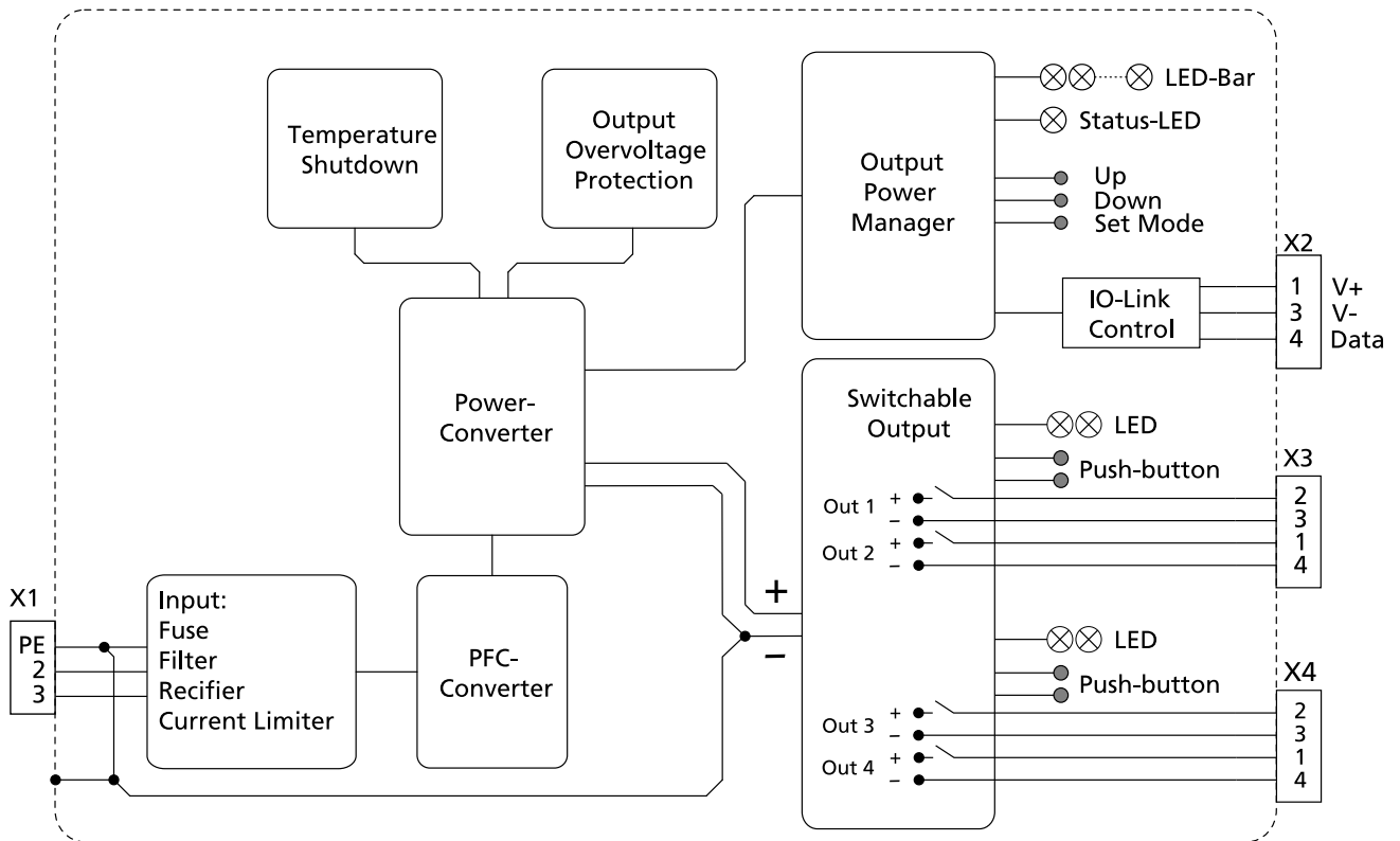
Fig. 12-1: Functional Diagram FPH500.245-047-154
