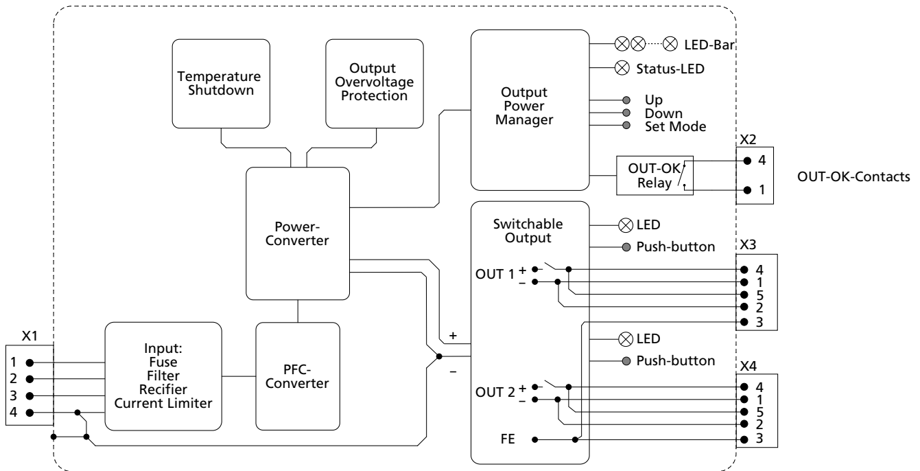
Fig. 12-1: Functional Diagram FPT500.245-053-113
