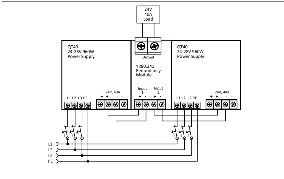
Fig. 25-1 Typical 1+1 Redundant configuration for 40A with a dual redundancy module
