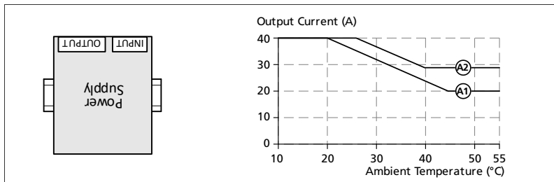
Fig. 26-11 Mounting Orientation B (Upside down)
