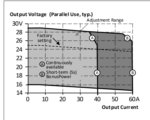
Fig. 6-2 Output voltage vs. output current in "parallel use" mode, typ.
