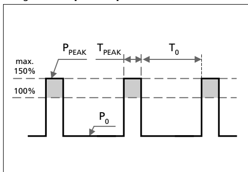
Fig. 26-1 Repetitive pulse loads, definitions
