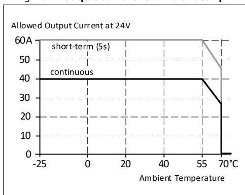
Fig. 18-1 Output current vs. ambient temp.
