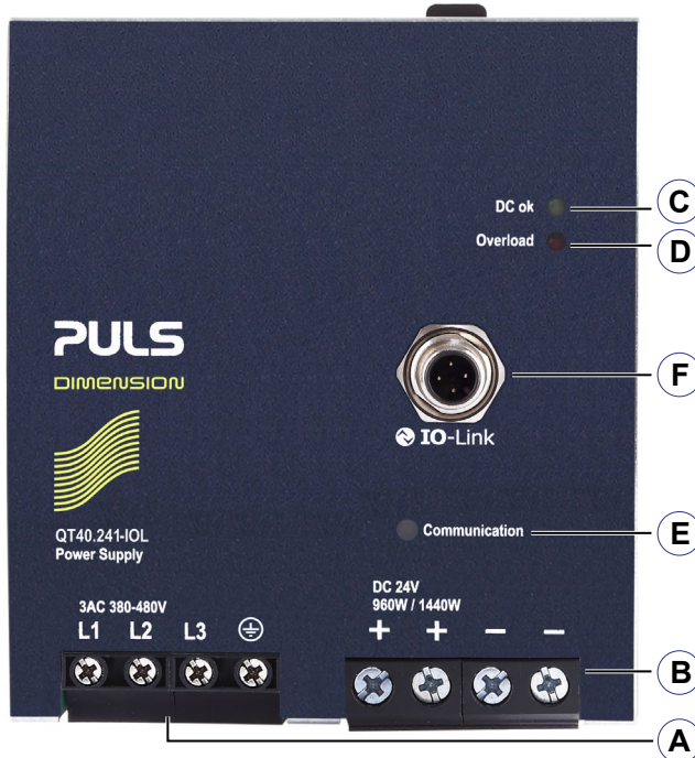
Fig. 16-1 Front side
