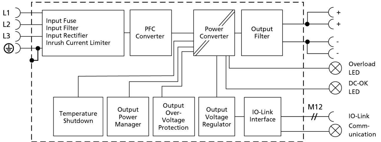
Fig. 14-1 Functional diagram
