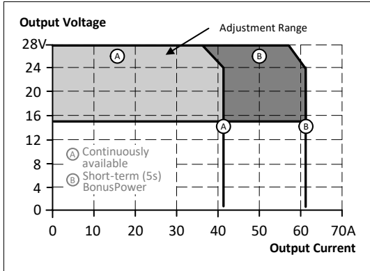
Fig. 6-1 Output voltage vs. output current in "single use" mode, typ.
