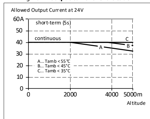
Fig. 18-2 Output current vs. altitude
