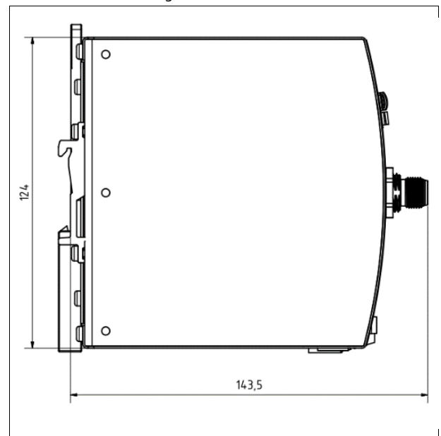
Fig. 24-2 Side view
