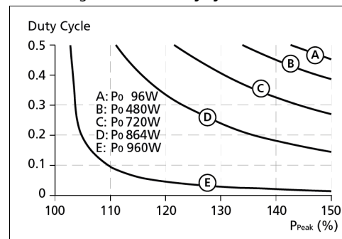
Fig. 26-2 Max. duty cycle curve
