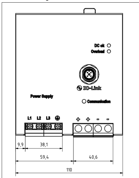
Fig. 24-1 Front view
