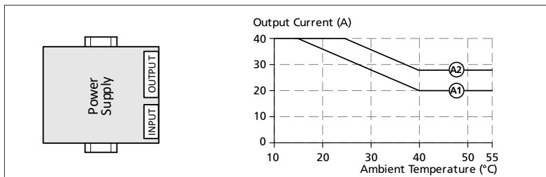
Fig. 26-14 Mounting Orientation E (Horizontal ccw)
