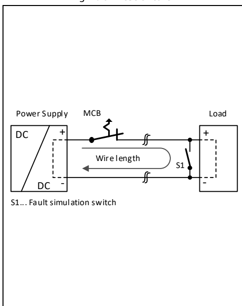
Fig. 26-9 Test circuit
