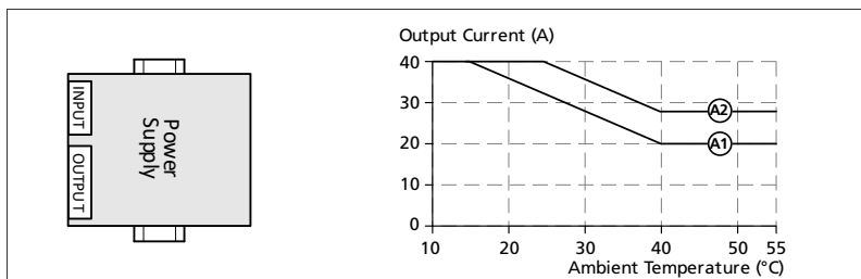
Fig. 26-13 Mounting Orientation D (Horizontal cw)
