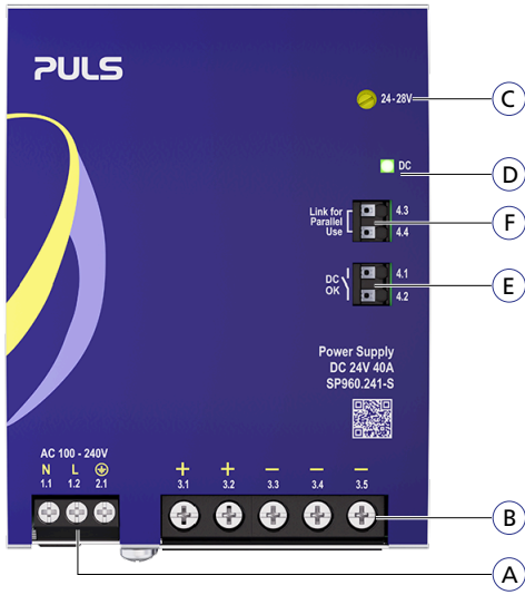
Fig. 15-1: Front side
