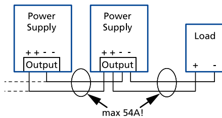
Fig. 14-1: Daisy chaining of outputs
