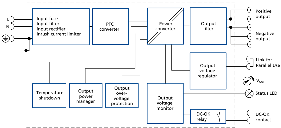
Fig. 13-1: Functional Diagram SP960.241-S
