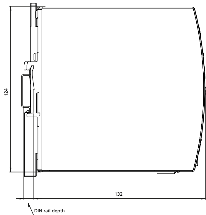
Fig. 23-2: Side view
