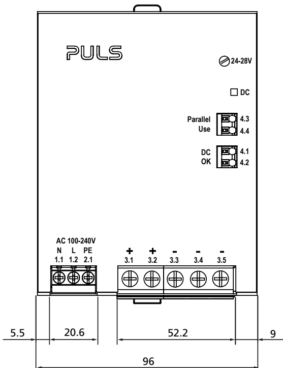
Fig. 23-1: Front view
