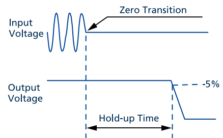
Fig. 8-2: Shut-down behaviour
