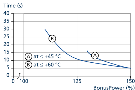
Fig. 7-1: Calculated time availability of BonusPower up to +60 °C
