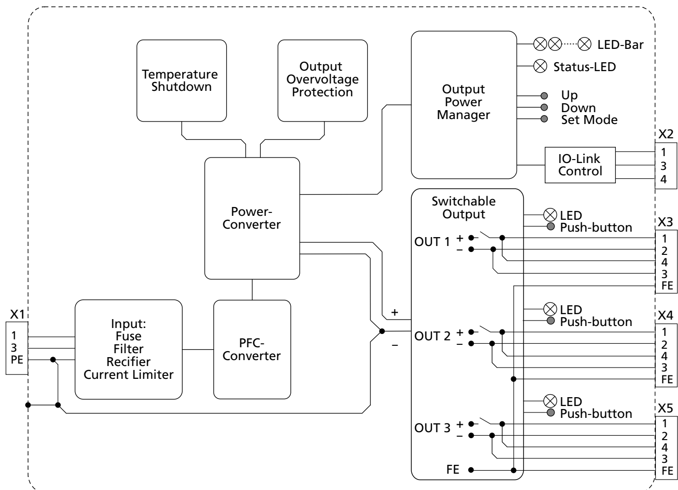
Fig. 12-1: Functional Diagram FPS300.246-036-104
