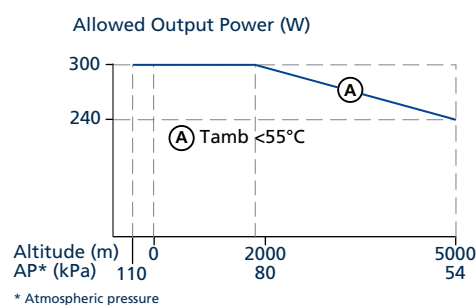
Fig. 16-2: Output power vs. altitude
