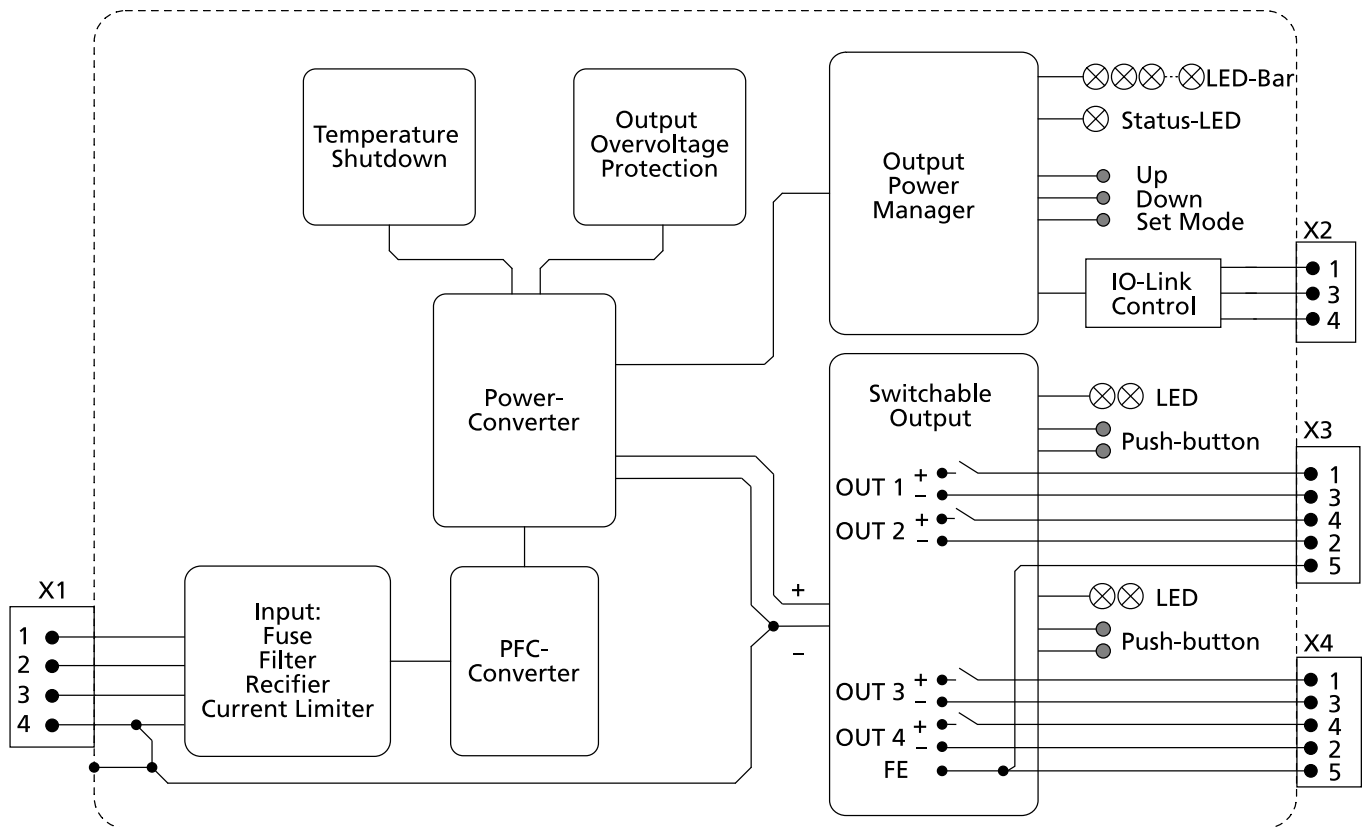
Fig. 12-1: Functional Diagram FPT500.245-034-105
