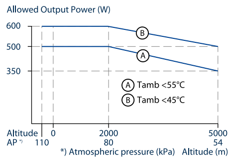
Fig. 16-2: Output power vs. altitude
